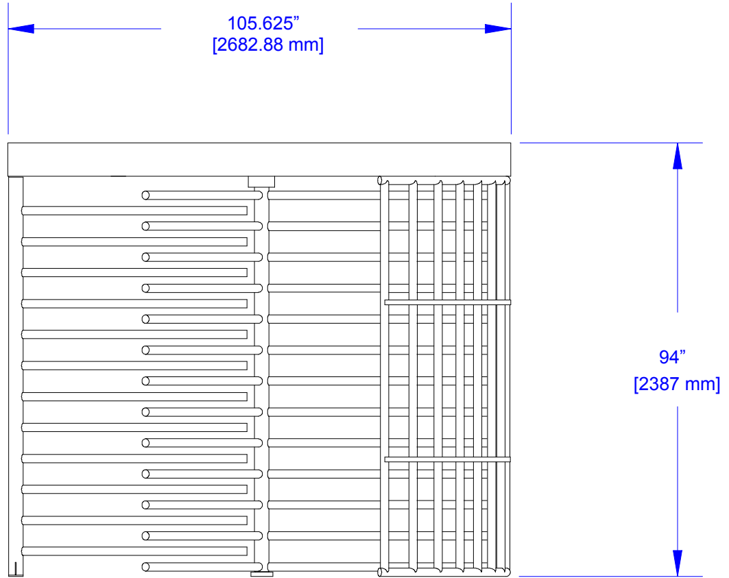
ELEVATION VIEW
