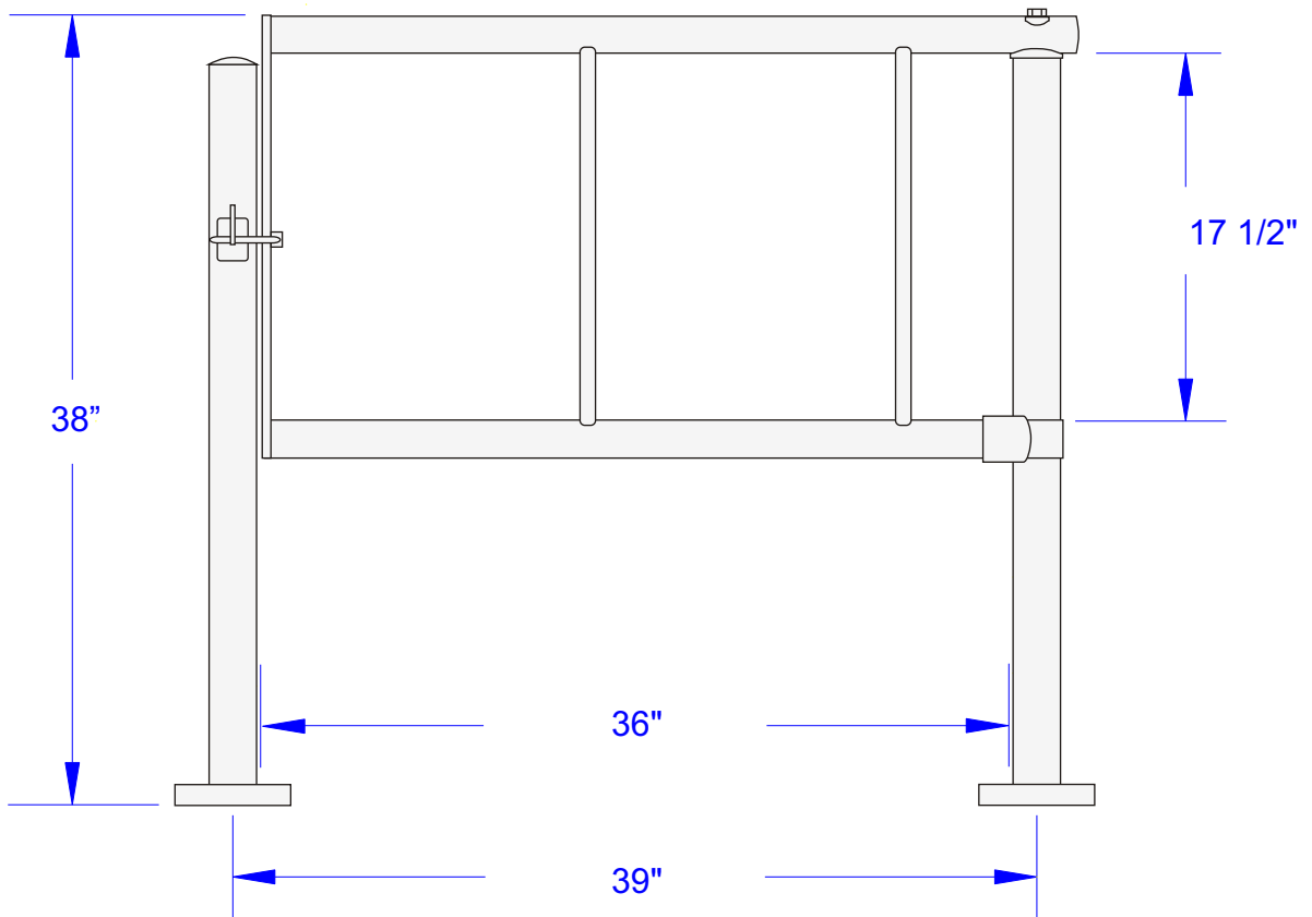
ELEVATION VIEW
