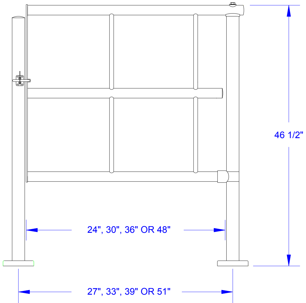
ELEVATION VIEW
