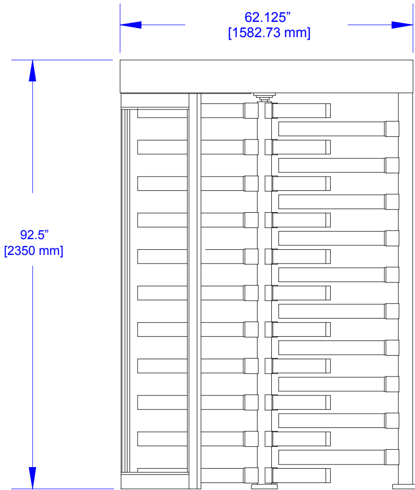
ELEVATION VIEW
