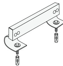
Heavy duty 1" bolts and double expansion anchors provide installation stability.
