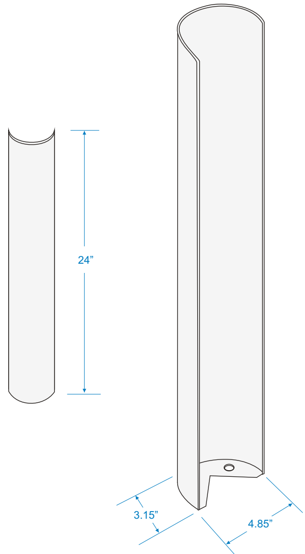
Model DM Dimensions
